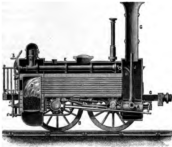
FIG. 57.—Stephenson's Locomotive, 1825.
